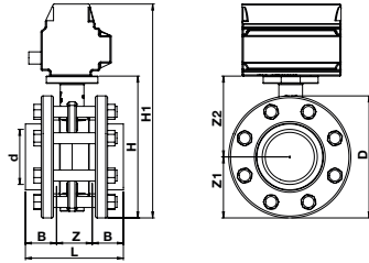
304 Paslanmaz Civata-Somun-Pul / 304.S.S.Screw,Nut,Washer
